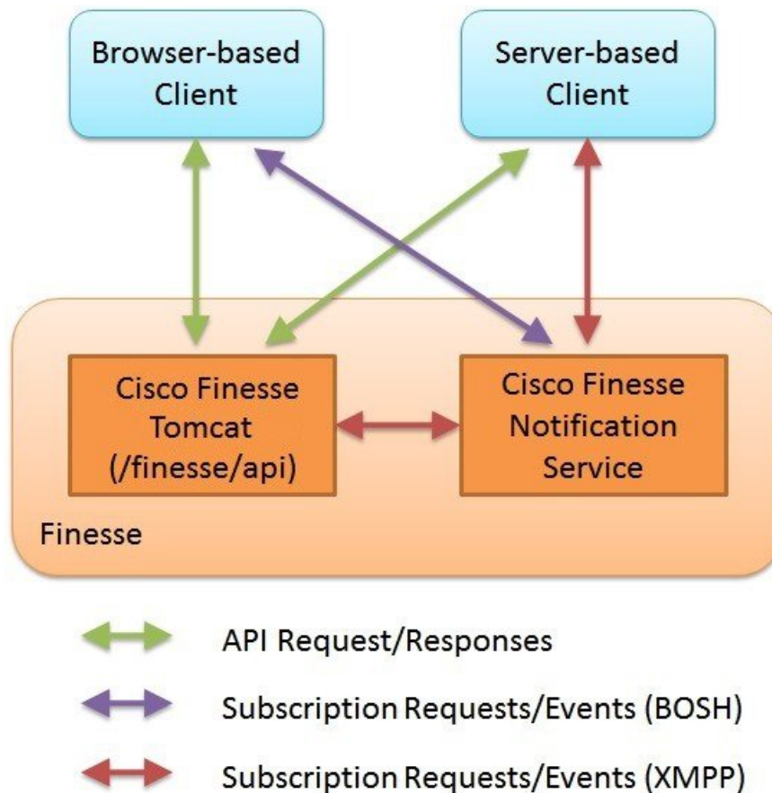
Figure 1: Finesse API and Event Flow
