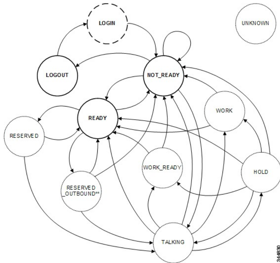
Figure 8: Supported State Transitions by Agent (Unified CCE)
